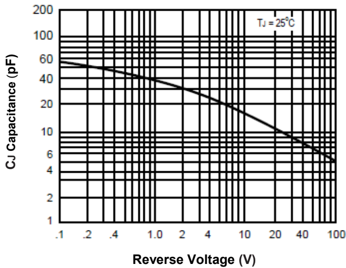
Fig.5- Junction Capacitance
