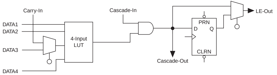
Figure 6. FLEX 8000 LE Operating Modes
