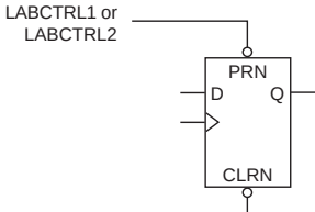
Figure 7. FLEX 8000 LE Asynchronous Clear & Preset Modes
