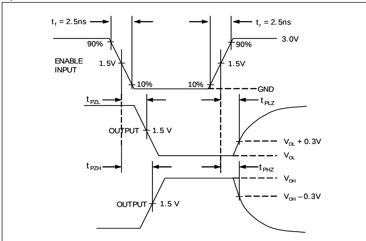
Figure 6. AC Waveforms
