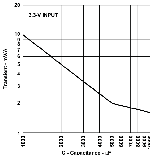
Figure 11. Capacitor Type B, 1000 < C(\mu\text{F}) \times \text{ESR}(\text{m}\Omega) \leq 5000 (e.g. Polymer-Tantalum)
