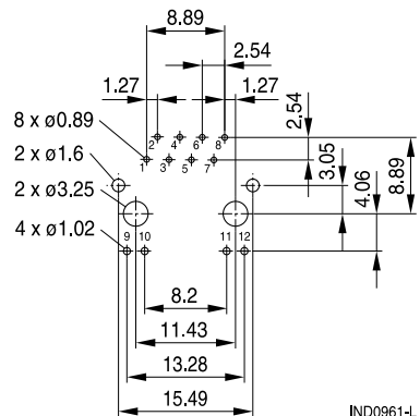
Layout recommendation (top view)
