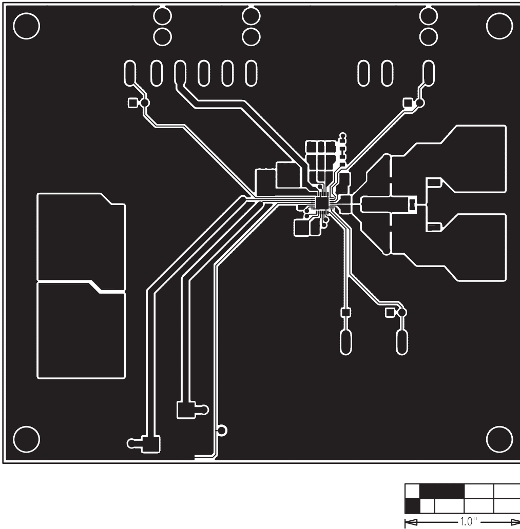
Figure 3. MAX9792A EV Kit PCB Layout—Component Side
