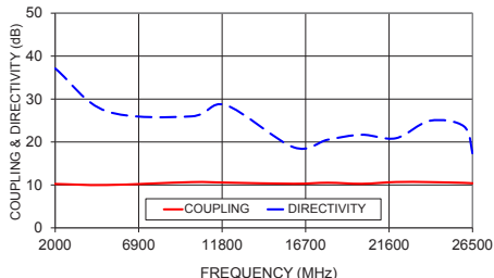
ZCDC10-02263S+ COUPLING & DIRECTIVITY
