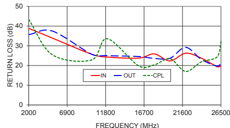
ZCDC10-02263S+ RETURN LOSS
