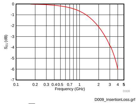
图 11. Insertion Loss
