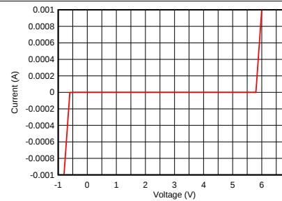
图 6. DC IV-Curve, I/O Pin to GND
