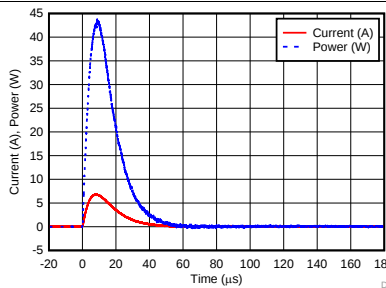
图 5. Surge Curve (IEC 61000-4-5, t_p = 8/20 \mu s), I/O Pin to GND
