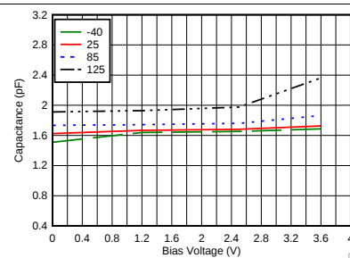
图 8. Capacitance Vs. Bias Voltage at Different Temperatures (°C)
