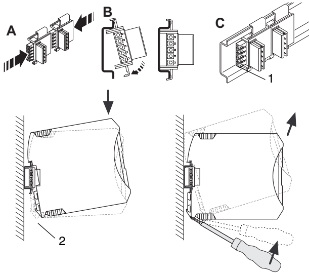
Figure 4 Assembly and removal
