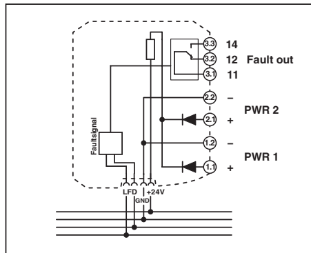
Figure 1 Basic circuit diagram with connection terminal blocks
