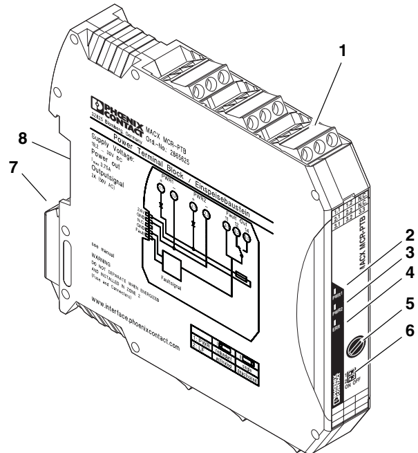
Figure 2 Design
