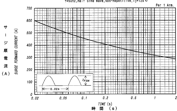
サージ順電流定格 SURGE CURRENT RATINGS f=50Hz, Half Sine Wave, Non-Repetitive, T_j = 125^\circ\text{C}
