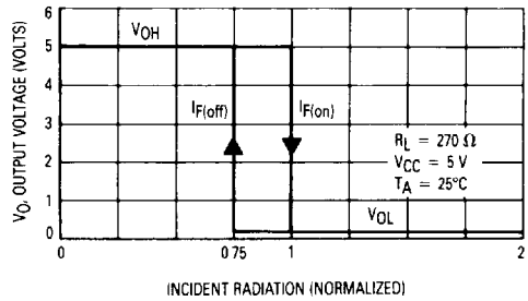
Figure 1. Transfer Characteristics
