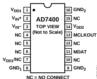
Figure 5. Pin Configuration
