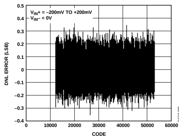
Figure 10. Typical DNL, \pm 200 mV Range (Using Sinc 3 Filter, 256 Decimation Rate)
