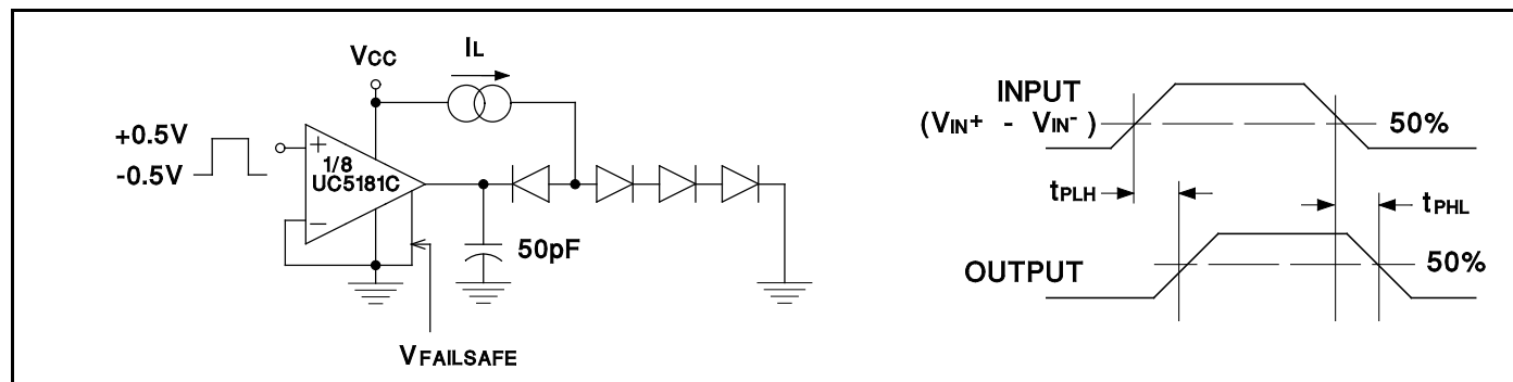
Figure 2. AC Test Circuit
