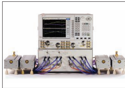
The N5262A millimeter-wave test-set controller connects four millimeter-wave test modules to the PNA-X. For two-port measurements, the N5261A millimeter-wave test-set controller is available.
