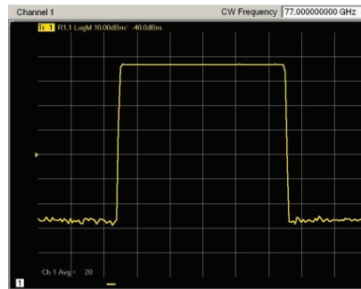
Pulse profile at 77 GHz using the internal pulsed source and IF gates of the PNA-X.
