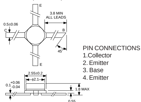
PACKAGE OUTLINE 18 RECOMMENDED P.C.B. LAYOUT
