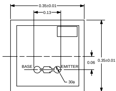
PACKAGE OUTLINE 18
