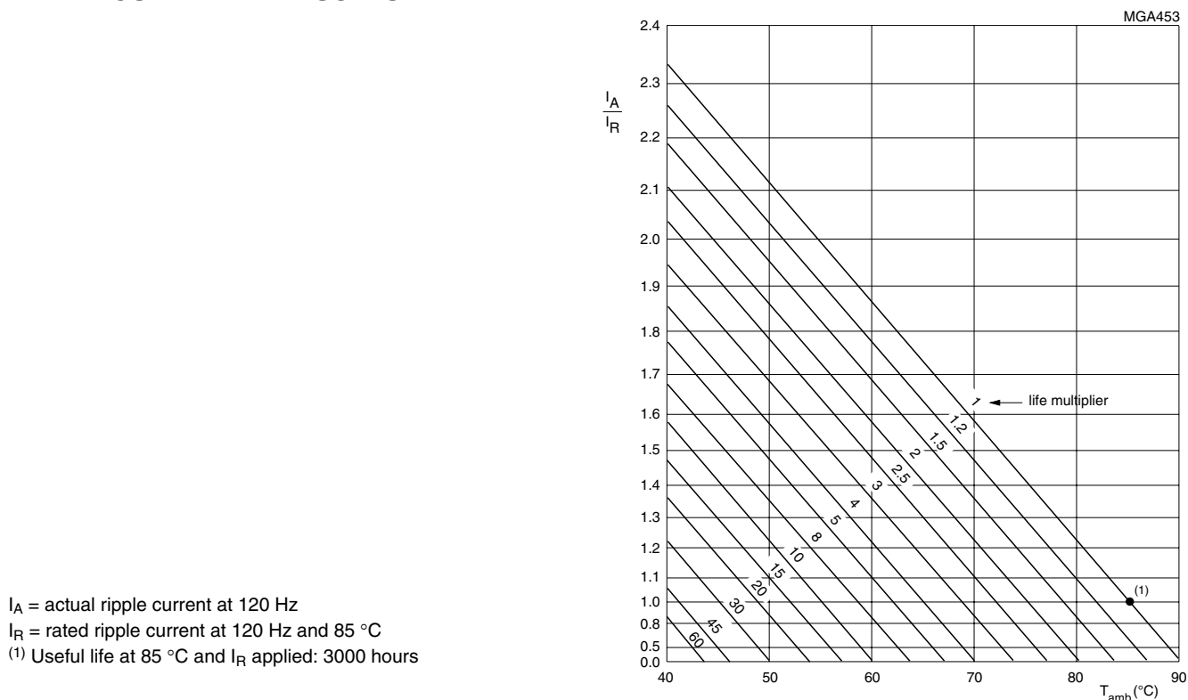
Fig.4 Multiplier of useful life as a function of ambient temperature and ripple current load
