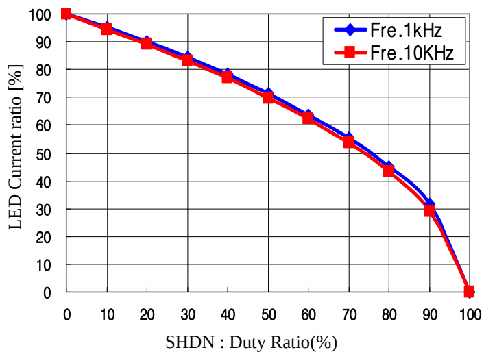
Fig.7 Dimming Curve
