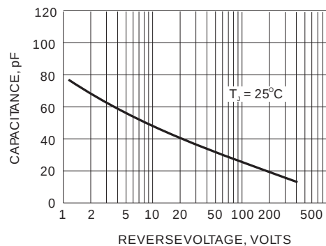
Fig.5-TYPICAL JUNCTION CAPACITANCE
