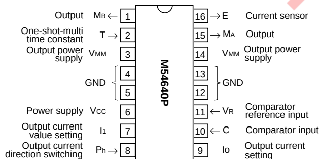
Outline 16P4
