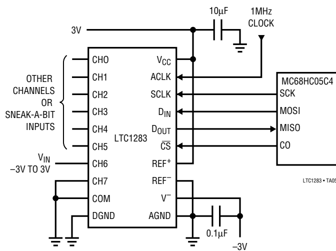
SNEAK-A-BIT Circuit
