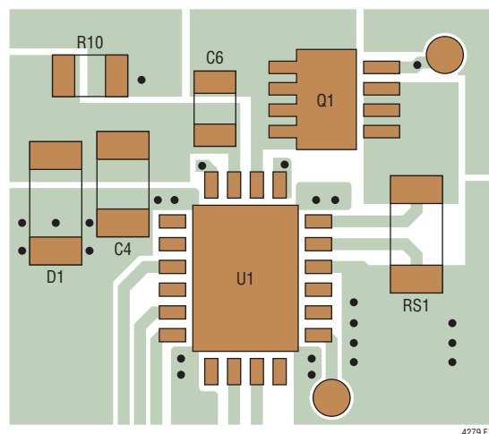
Figure 14. Example LTC4279 Layout
