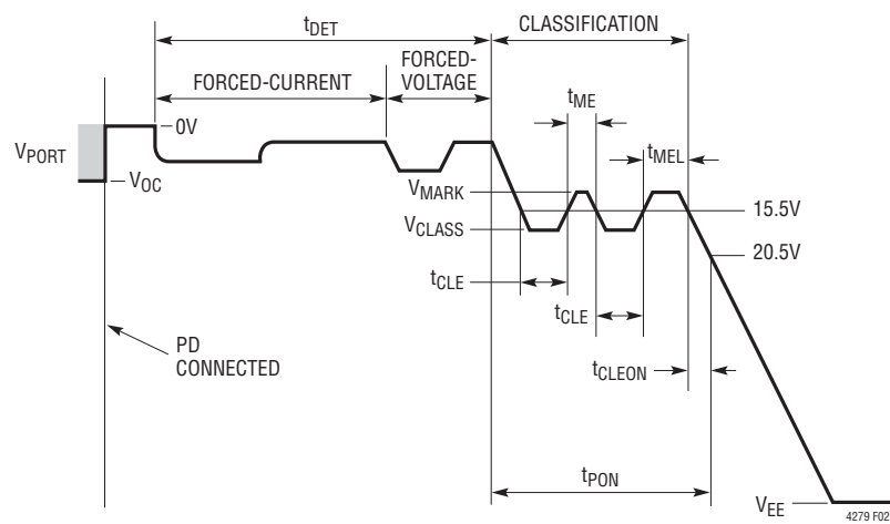
Figure 2. Detect, Two Event Class and Turn-On Timing
