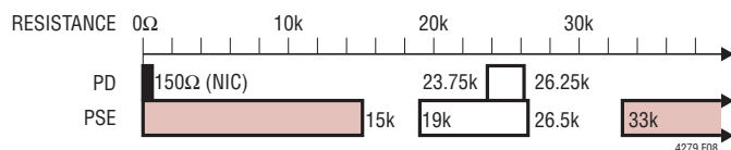
Figure 8. IEEE 802.3at Signature Resistance Ranges
