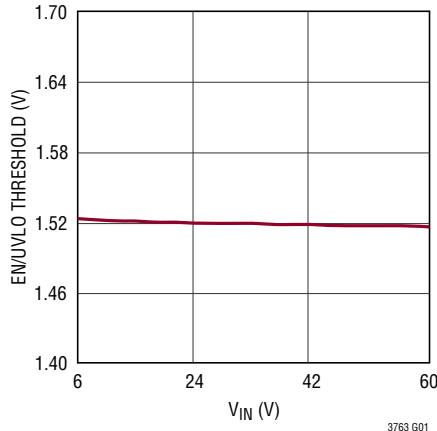
EN/UVLO Threshold (Falling)
