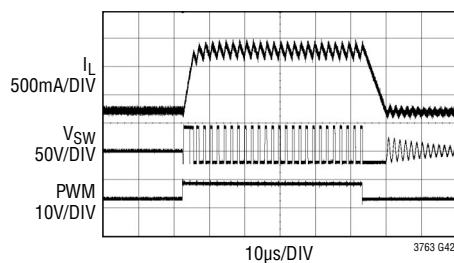
PWM Dimming
