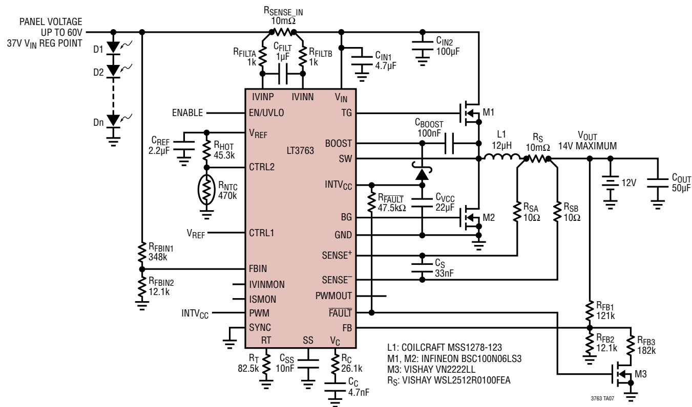
Solar Powered SLA Battery Charging
