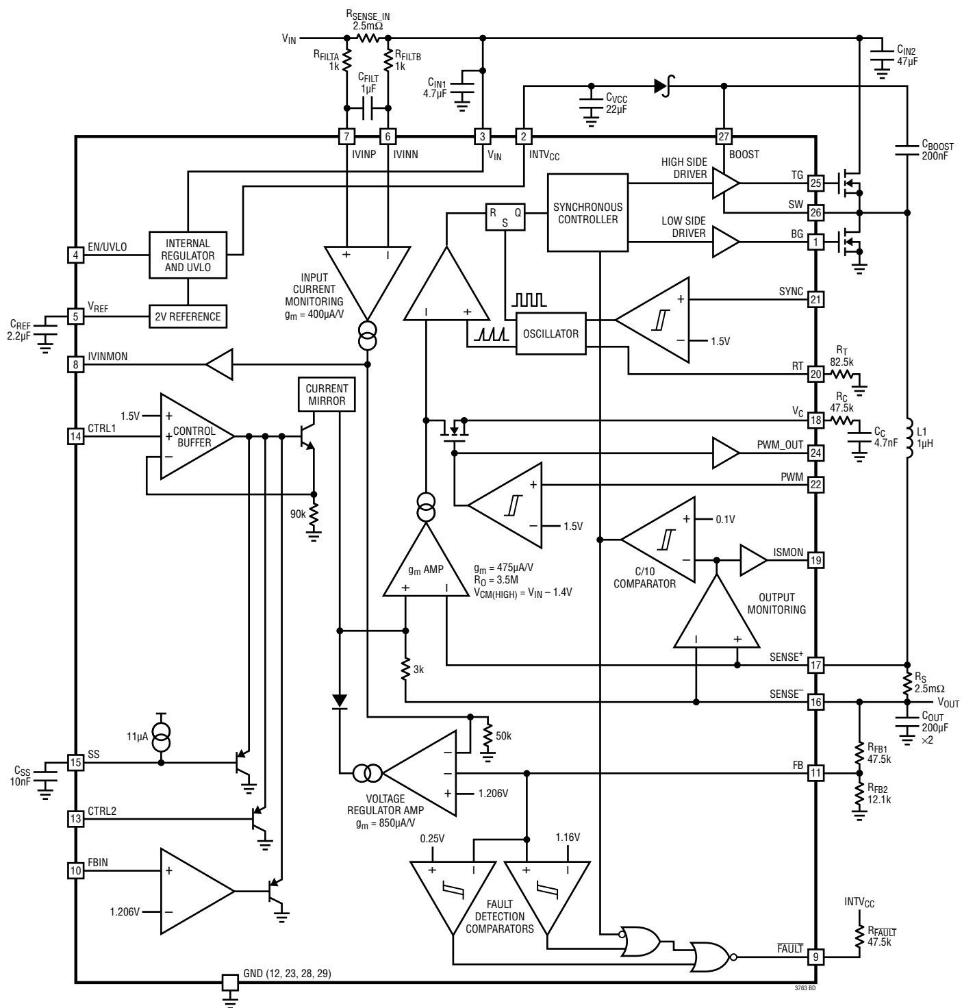
Figure 1. Block Diagram
