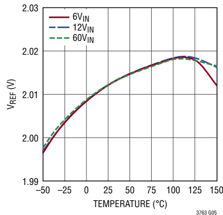
VREF Voltage
