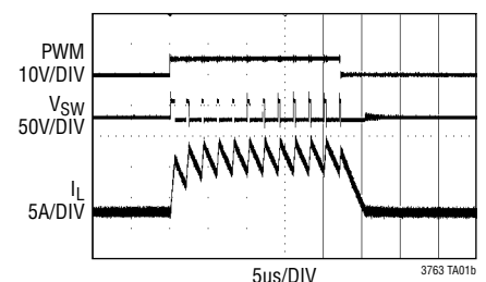
PWM Dimming
