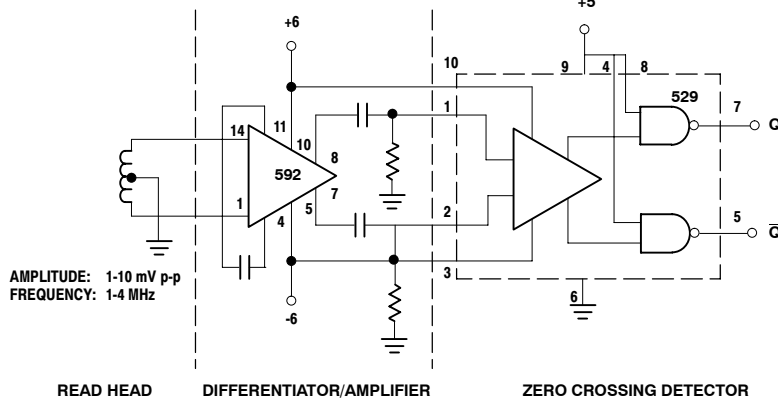
Disc/Tape Phase-Modulated Readback Systems
