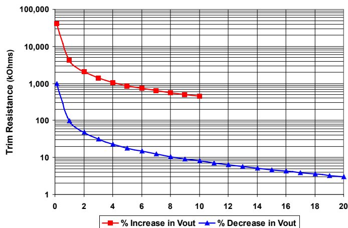
Figure C: Trim Graph for 52.5Vout module
