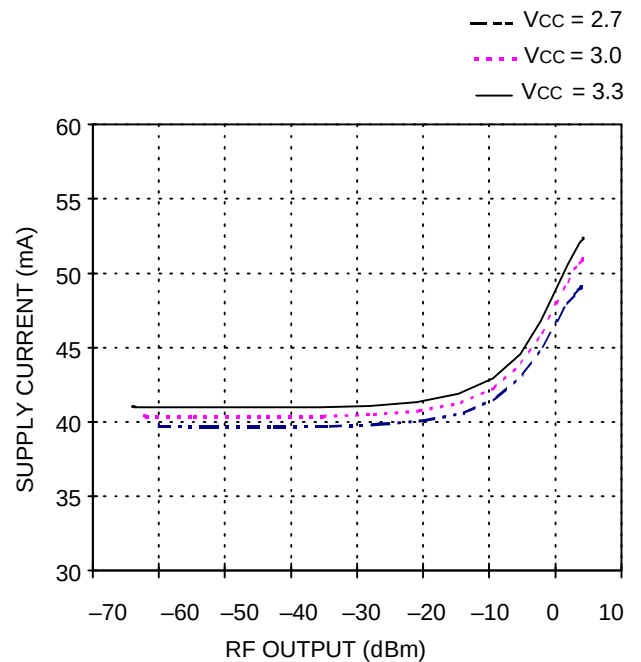
Figure 9. Supply Current vs. Output Power
