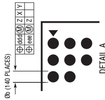
DETAIL B PACKAGE SIDE VIEW
