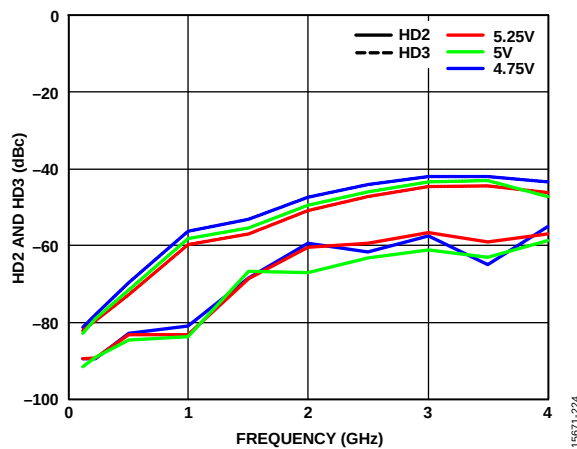
Figure 24. HD2 and HD3 vs. Frequency for Various Supplies
