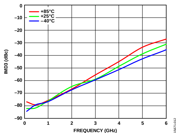
Figure 12. IMD3 vs. Frequency over Temperature
