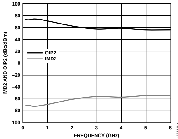
Figure 14. Second-Order Intermodulation Distortion (IMD2) and Output Second-Order Intercept (OIP2) vs. Frequency
