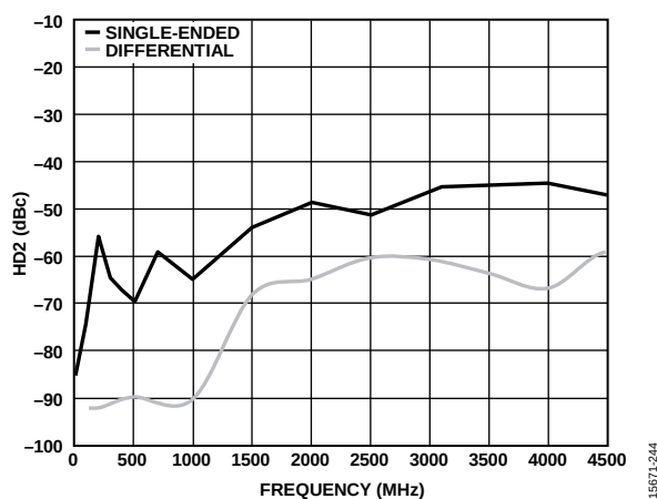
Figure 44. HD2 for Single-Ended and Differential Configurations vs. Frequency, V_{OUT} = 2\text{ V p-p}
