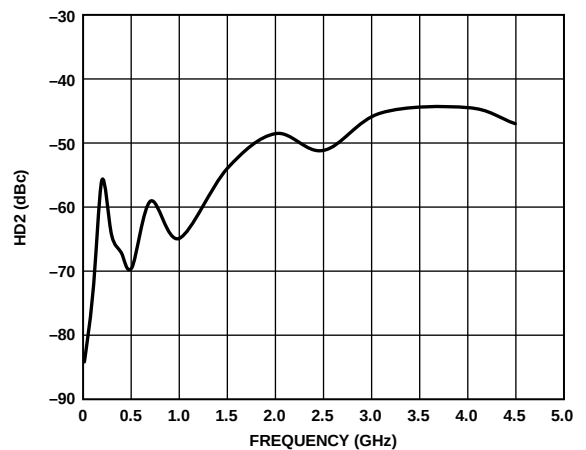
Figure 26. HD2 vs. Frequency for a Single-Ended Input Circuit
