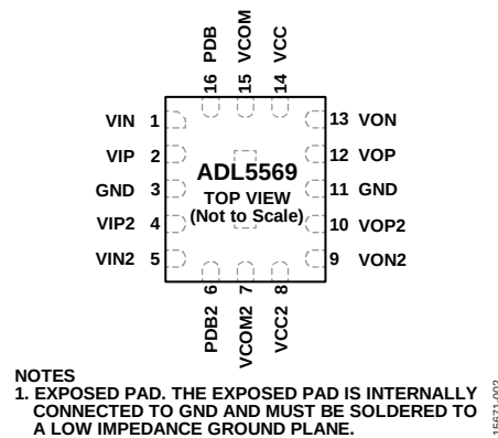
Figure 2. Pin Configuration
