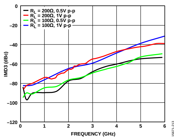
Figure 13. IMD3 vs. Frequency over R_{LOAD} for P_{OUT} per Tone
