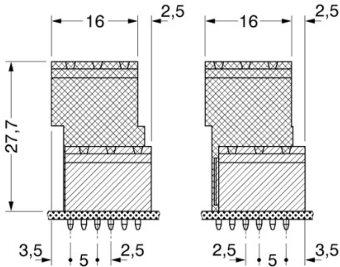
Dimensioned drawing
