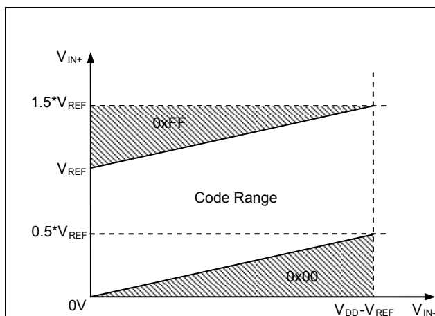
Figure 6: Input voltage range in unipolar mode
