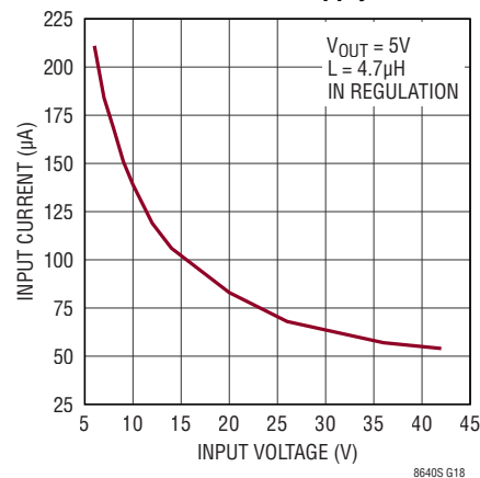
LT8643S No-Load Supply Current
