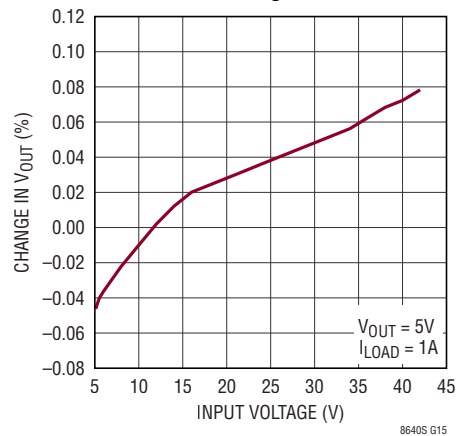
LT8640S Line Regulation
