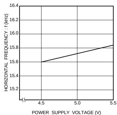
Fig. 13 Horizontal free-running frequency vs. power supply voltage
