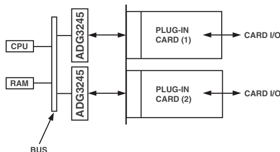
Figure 12. ADG3245 in a Hot Plug Application
