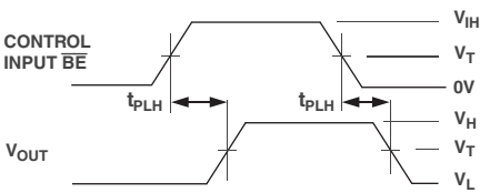
Figure 2. Propagation Delay
