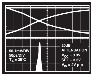
TPC 22. Jitter @ 1.244 Gbps, PRBS 31
