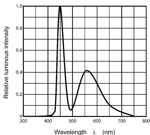
Fig. 8.6 Wavelength Characteristic
