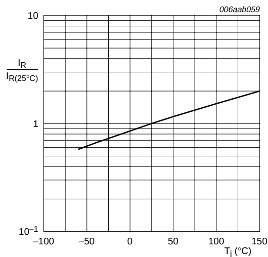
PESD5Z2.5; V_{RWM} = 2.5 \text{ V} PESD5Z3.3; V_{RWM} = 3.3 \text{ V} I_R is less than 50 nA at 150 ^\circ\text{C} for: PESD5Z5.0; V_{RWM} = 5.0 \text{ V} PESD5Z6.0; V_{RWM} = 6.0 \text{ V} PESD5Z7.0; V_{RWM} = 7.0 \text{ V} PESD5Z12; V_{RWM} = 12.0 \text{ V}
