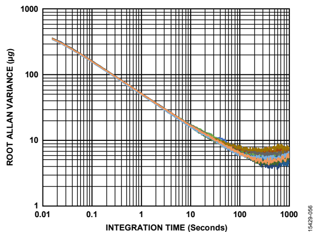
Figure 56. ADXL357 RAV, Y-Axis
