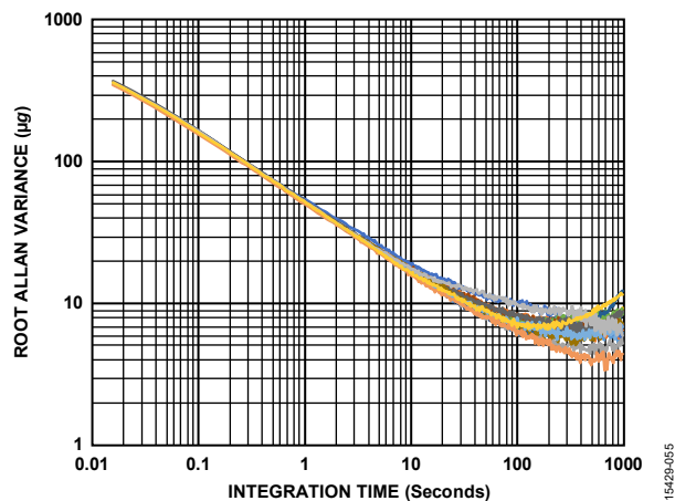
Figure 55. ADXL357 RAV, X-Axis
