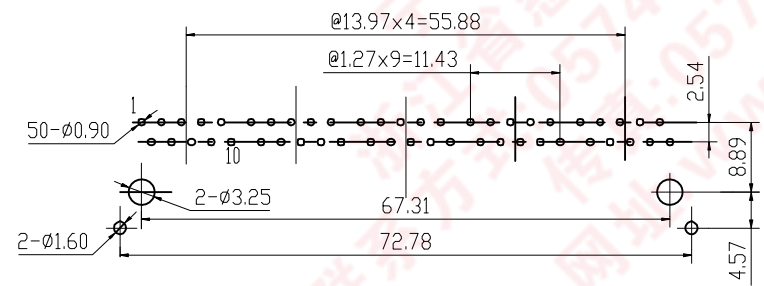
PC BOARD LAYOUT THICKNESS=1.6mm
