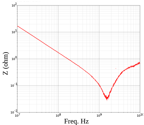
Figure 2 - 1nF UWSC measurement results (Impedance characteristic versus Frequency in shunt mode)
