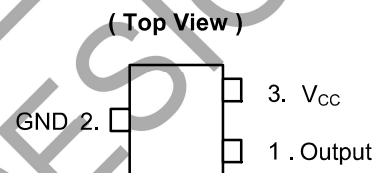
SC59R
