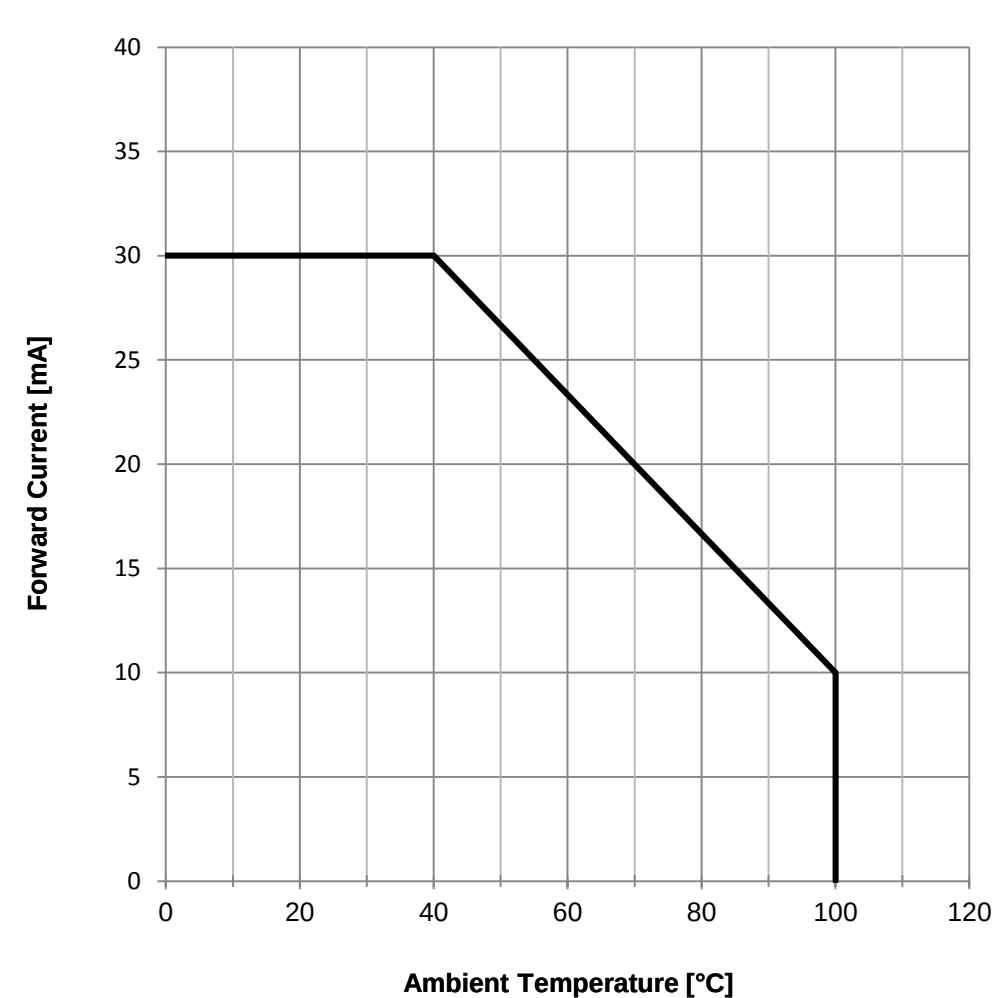
Derating Curve:
