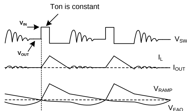
Figure 4: Light-Load Operation
