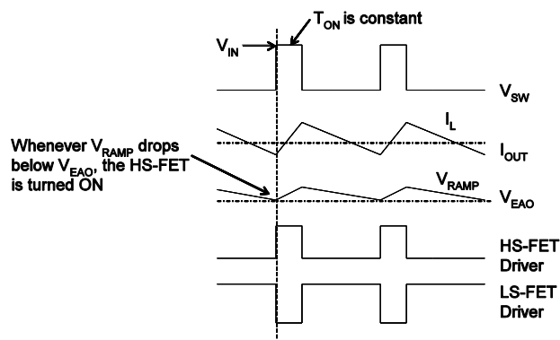
Figure 3: Heavy-Load Operation
