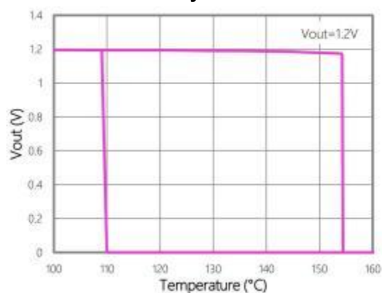
OTP Hysteresis
