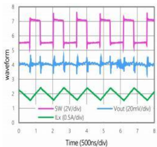
Switching Waveform
