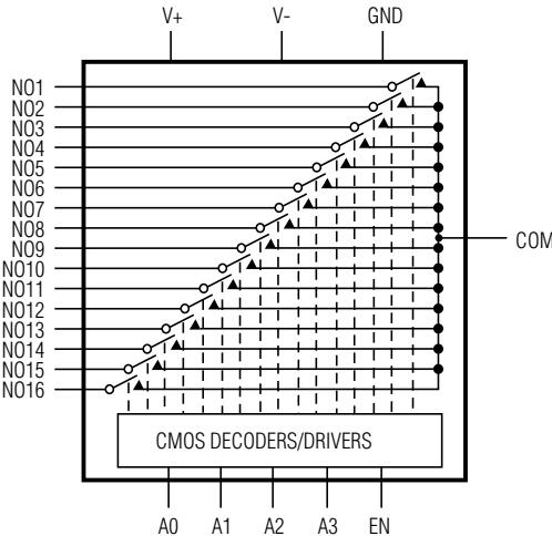
MAX306 16-CHANNEL SINGLE-ENDED MULTIPLEXER
