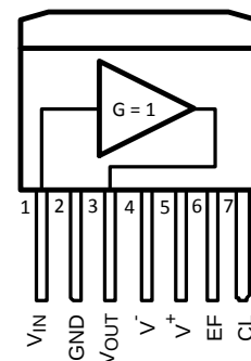
Figure 2. 7-Pin DDPACK(A)
