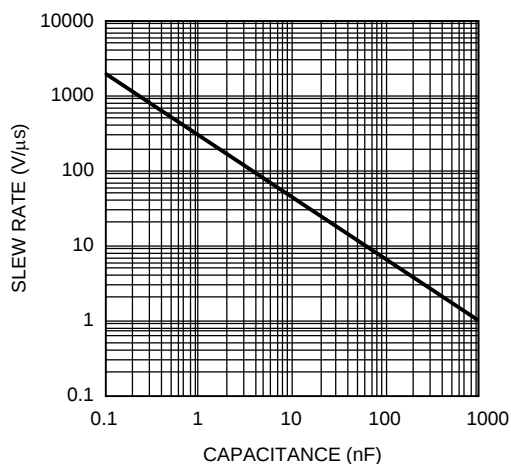
Figure 58. Slew Rate vs. Load Capacitance
