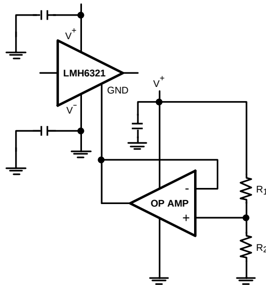
Figure 56. Using an Op Amp to Bias the GND Pin to \frac{1}{2} V^+ for Single Supply Operation
