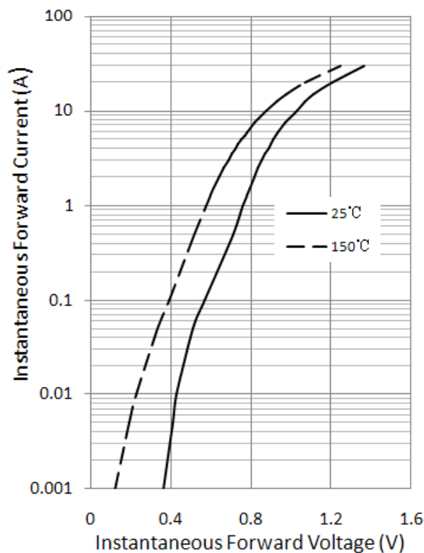
Figure 4. Typical Instantaneous Forward Characteristics
