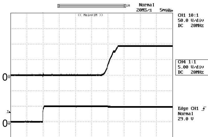
Figure 6: Turn-on transient at full rated load current (5 ns/div). Top Trace: Vout; 5V/div; Bottom Trace: Vin; 50V/div.
