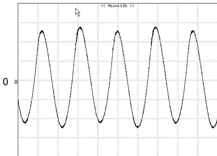
Figure 11: Input Terminal Ripple Current, i_c , at full rated output current and nominal input voltage with 10\mu\text{H} source impedance and 47\mu\text{F} electrolytic capacitor (200 mA/div, 2 \mu\text{s} /div).
