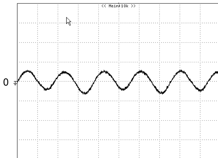
Figure 12: Input reflected ripple current, i_s , through a 10\mu\text{H} source inductor at nominal input voltage and rated load current (20 mA/div, 2 \mu\text{s} /div).
