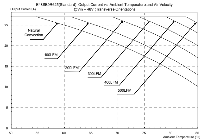
Figure 18: Output current vs. ambient temperature and air velocity @ V_{in}=48V (Transverse Orientation).
