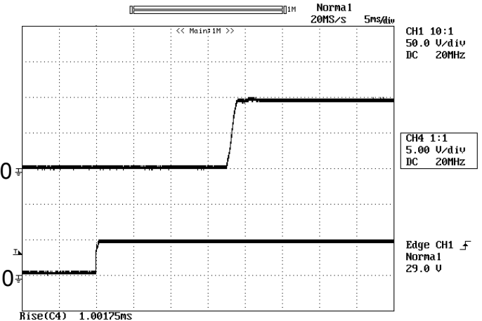
Figure 7: Turn-on transient at zero load current (5 ns/div). Top Trace: Vout; 5V/div; Bottom Trace: Vin; 50V/div.
