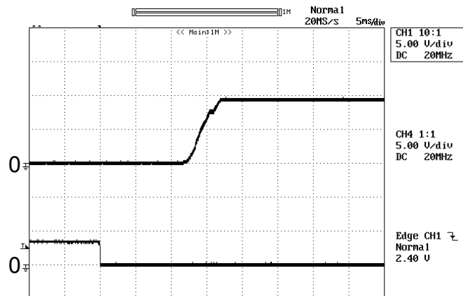
Figure 4: Turn-on transient at full rated load current (5 ns/div). Top Trace: Vout; 5V/div; Bottom Trace: ON/OFF input: 2V/div
