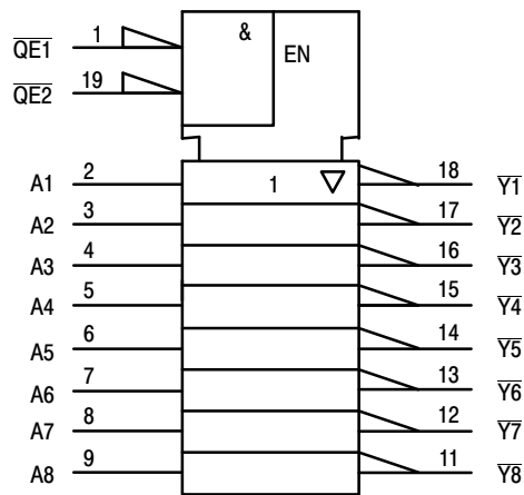
Figure 3. IEC LOGIC DIAGRAM
