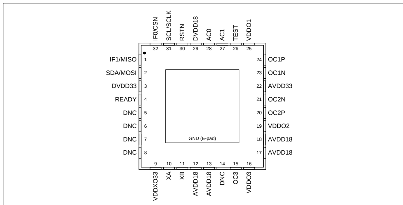
Figure 2 - Pin Diagram
