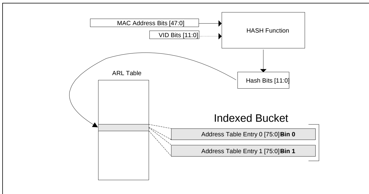
Figure 8: Mode Address Table Organization
