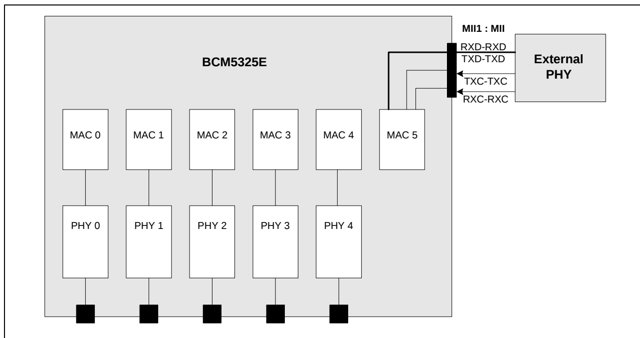
Figure 10: Normal MII Configuration
