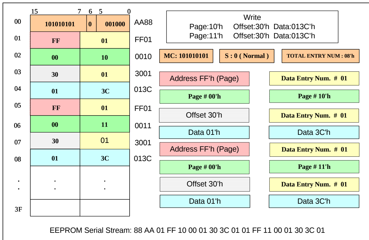
Figure 20: EEPROM Programming Example
