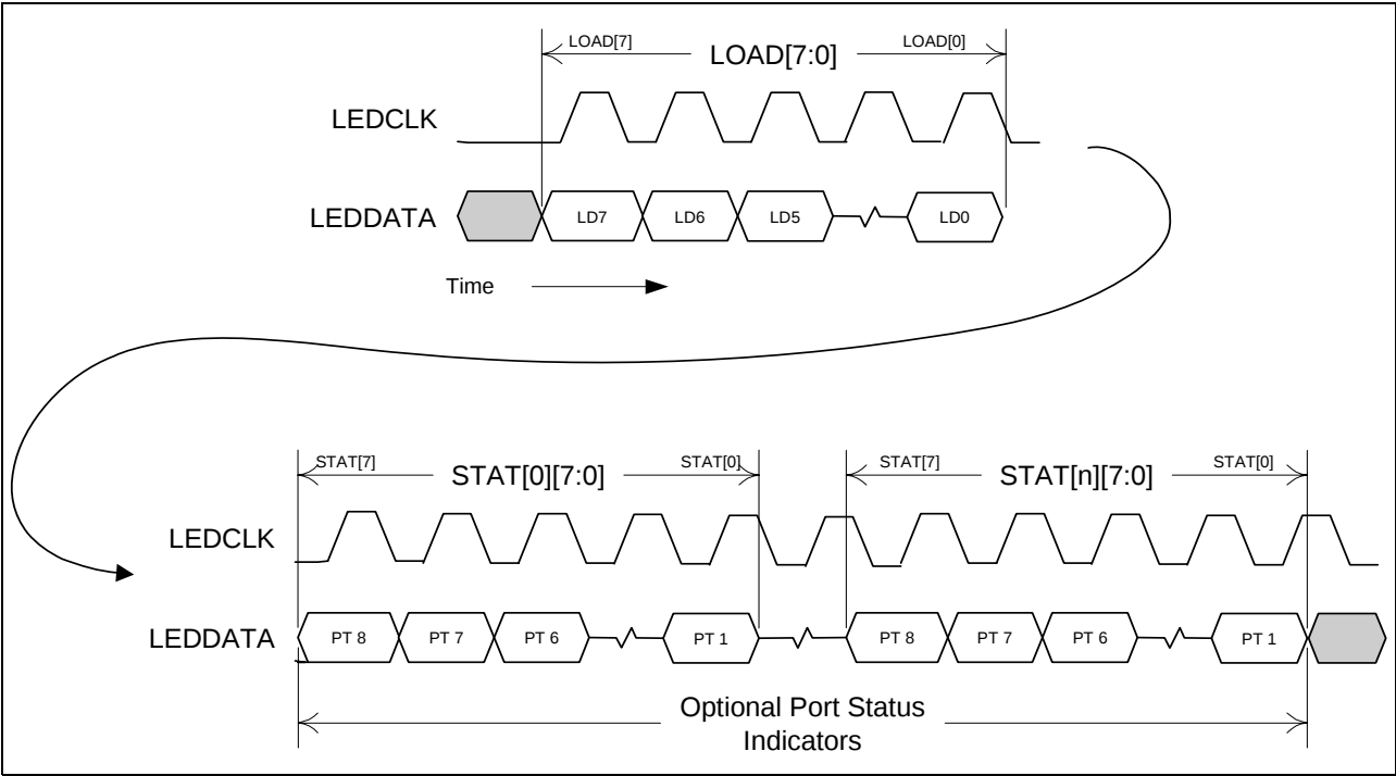
Figure 24: Serial LED Shift Sequence
