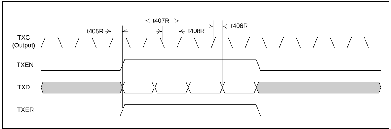
Figure 31: Reverse MII Mode Output Timings
