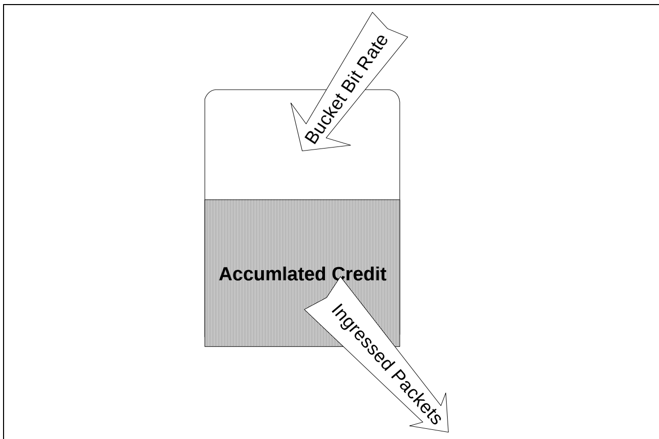
Figure 3: Bucket Flow
