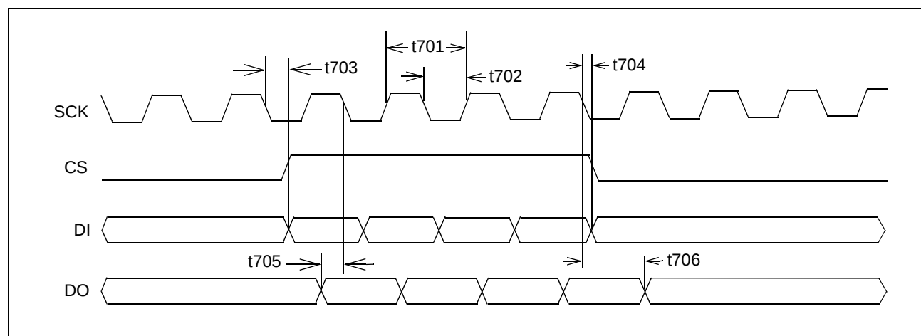
Figure 34: EEPROM Timing
