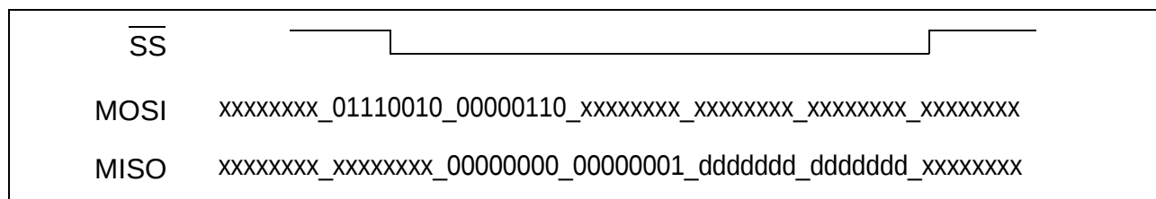
Figure 19: Timing Example
