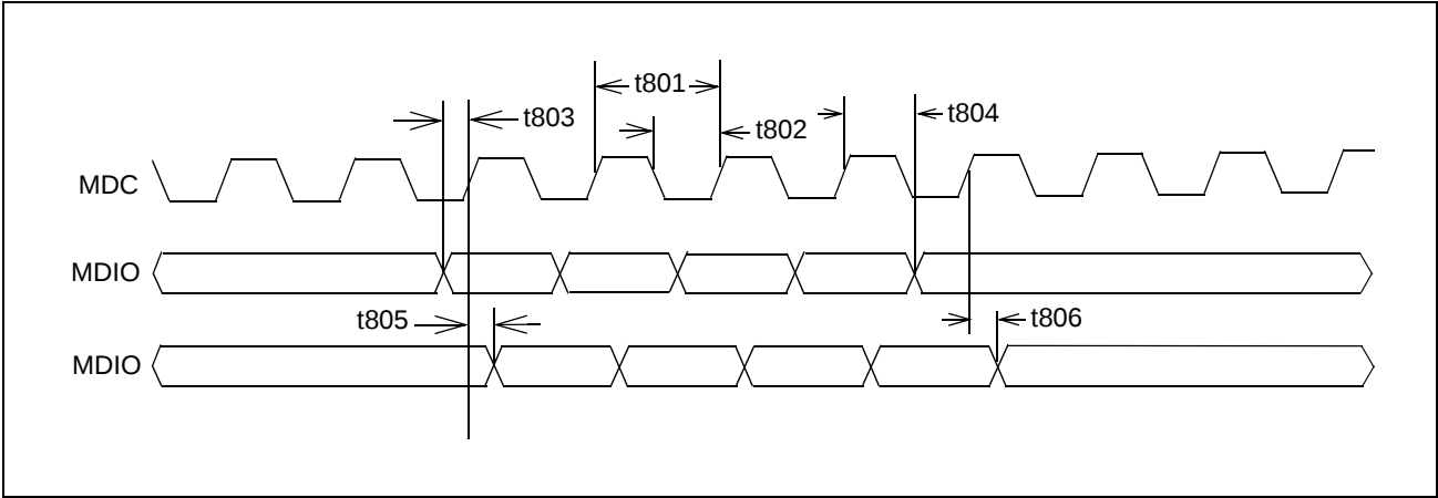
Figure 35: Management Data Interface (Slave Mode)
