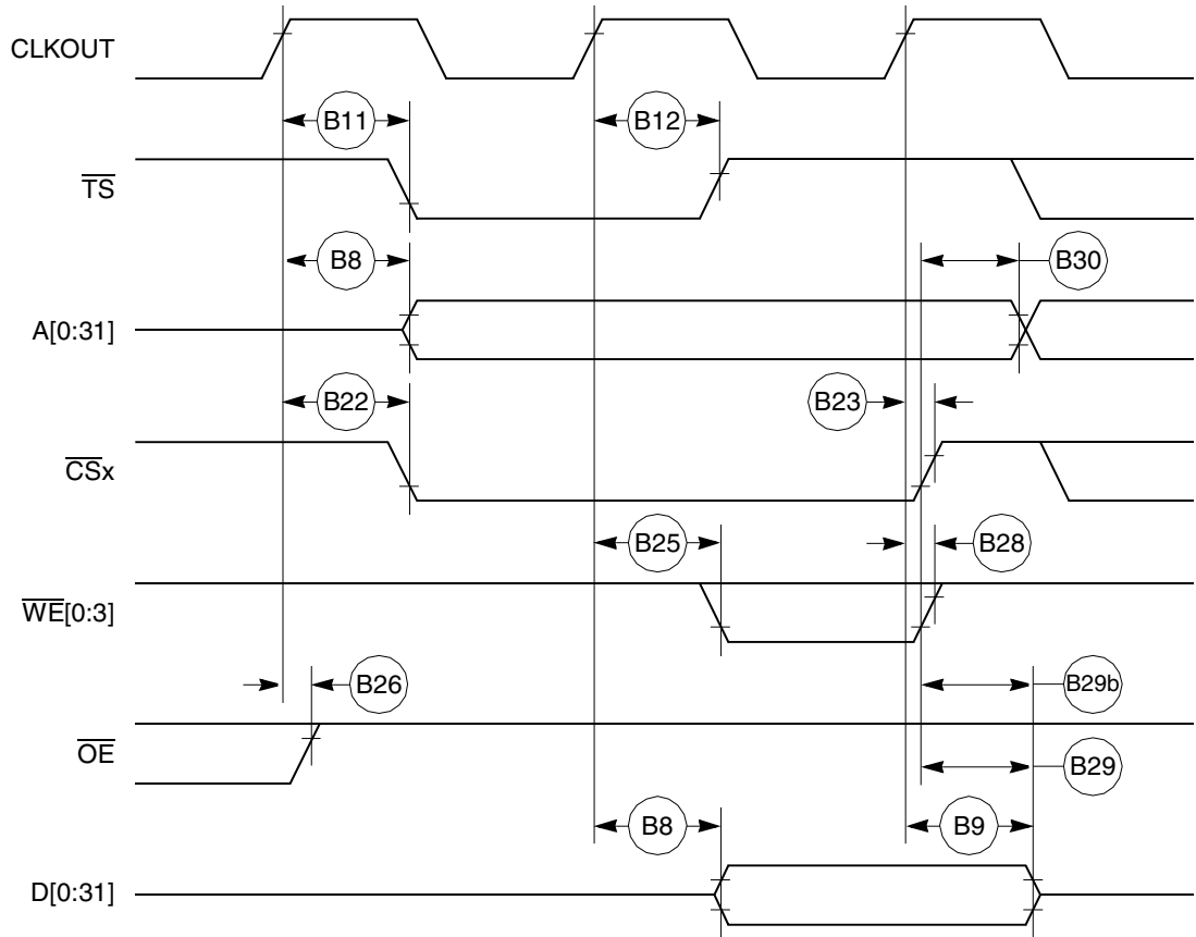
Figure 17. External Bus Write Timing (GPCM Controlled—TRLX = 0, CSNT = 0)
