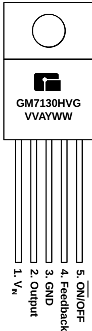
TO-220-5
