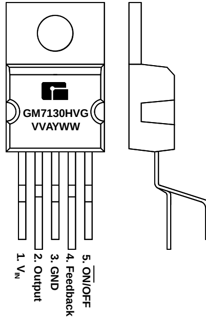
TO-220B-5
